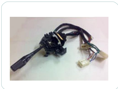
EOMC-79 MITSUBISHI CENTER Combination Switch Model- 4D31 Part No.- IB002892
