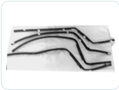
EOMC-109 MITSUBISHI CANTER Weather Strip Model- 4D31 Part No.- MB394614/5/6/7
