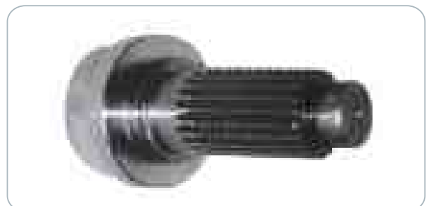
COUPLING SHAFT Z = 22 O.E.M. PART No. 346 410 99 99 PIPE Ø 98mm EOPPS-067 BEARING 60mm DIN 5480 60x55
