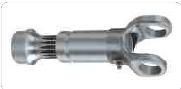
SLEEVE YOKE & TEETH Z = 16 O.E.M. PART No. 321 410 3402 U.J. CROSS Ø38mm EOPPS-064
