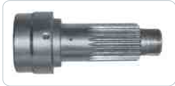
COUPLING SHAFT O.E.M. PART No. 336 410 99 99 EOPPS-069 Z = 26 PIPE Ø 90mm BEARING 55mm DIN 5482 55x50
