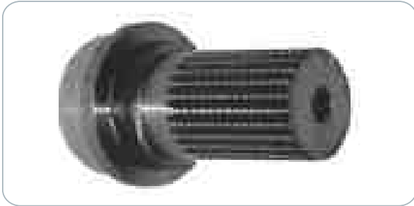
COUPLING SHAFT O.E.M. PART No. 395 410 99 99 EOPPS-068 Z = 26 PIPE Ø 98mm BEARING 70mm DIN 5480 70x65
